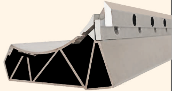
Sanmit Hardened Steel Knife with Machine Original Base
